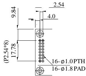
PIN DETAIL
