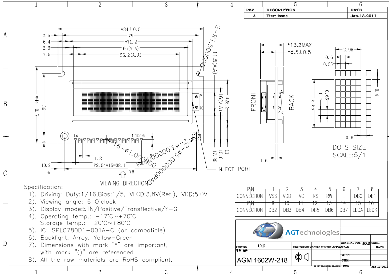
Figure 2. Dimensional outline
