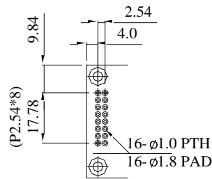
PIN DETAIL
