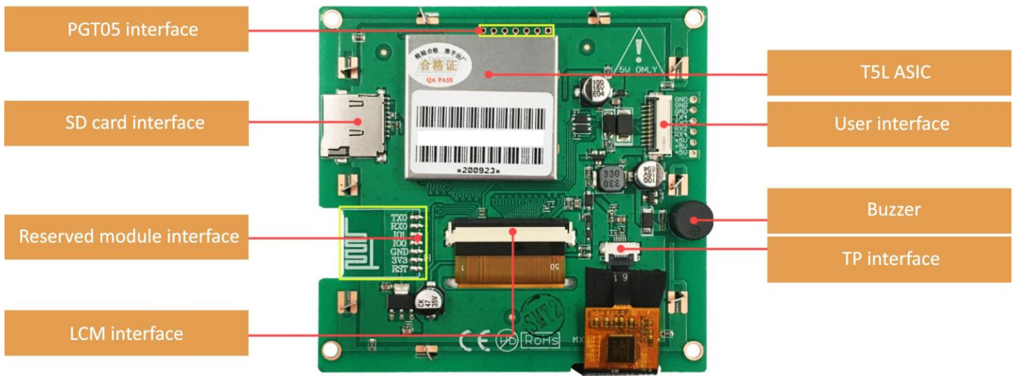
Hardware interface
