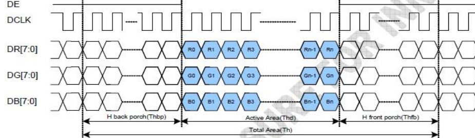
Parallel RGB input timign table
