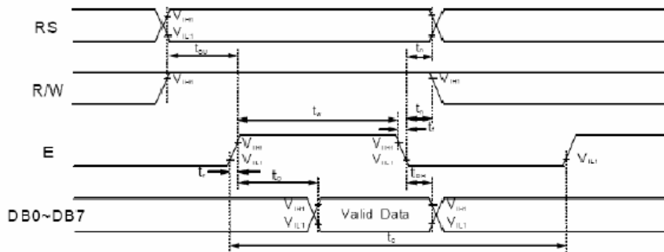
Figure 2 . Read Mode Timing Diagram
