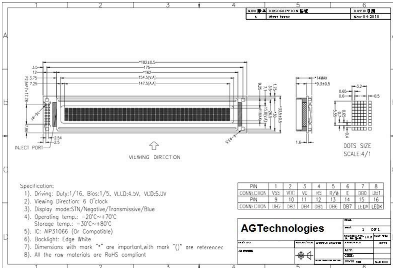
Figure 2. Dimensional Outline
