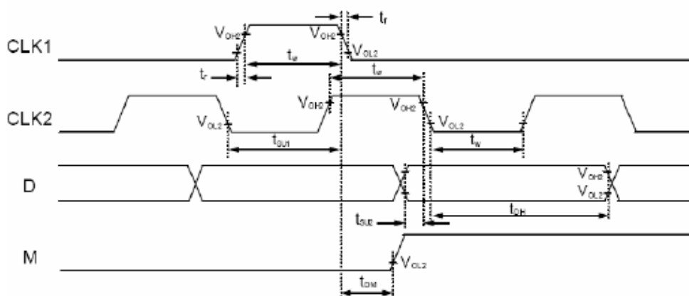
Figure 3 . Interface Mode With Extension Driver Timing Diagram
