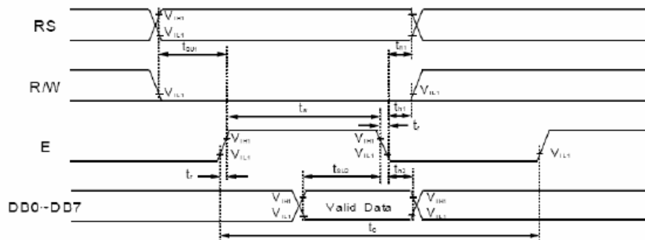
Figure 1 . Write Mode Timing Diagram
