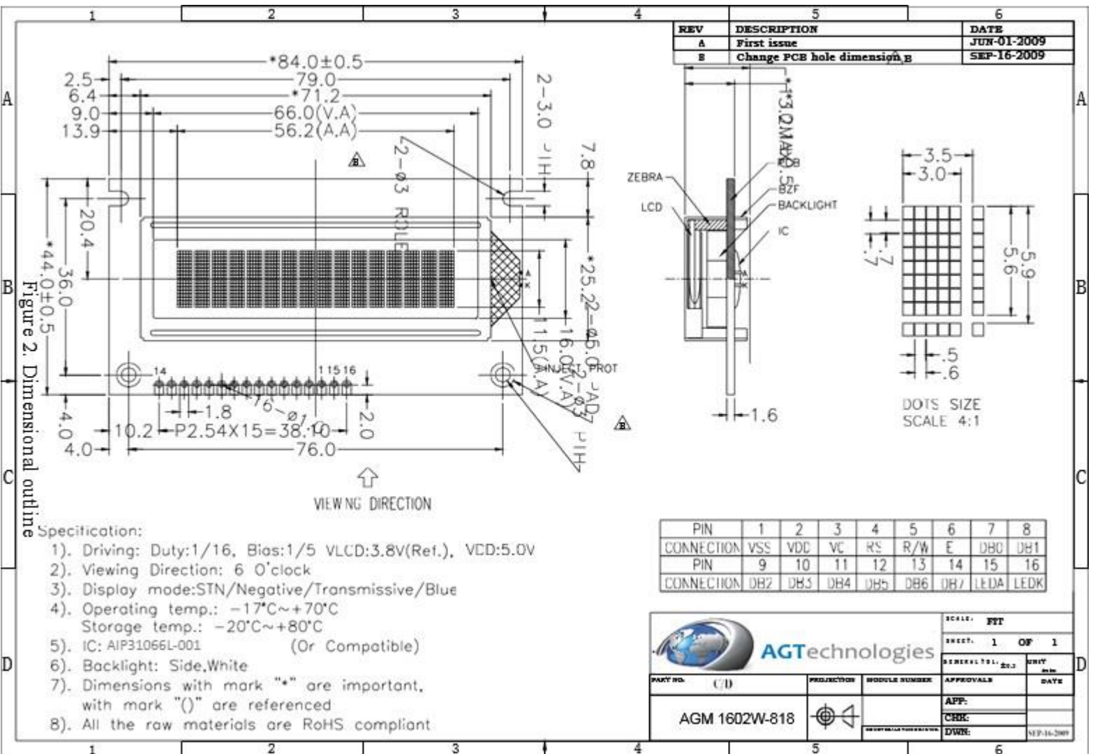
Figure 2. Dimensional outline
