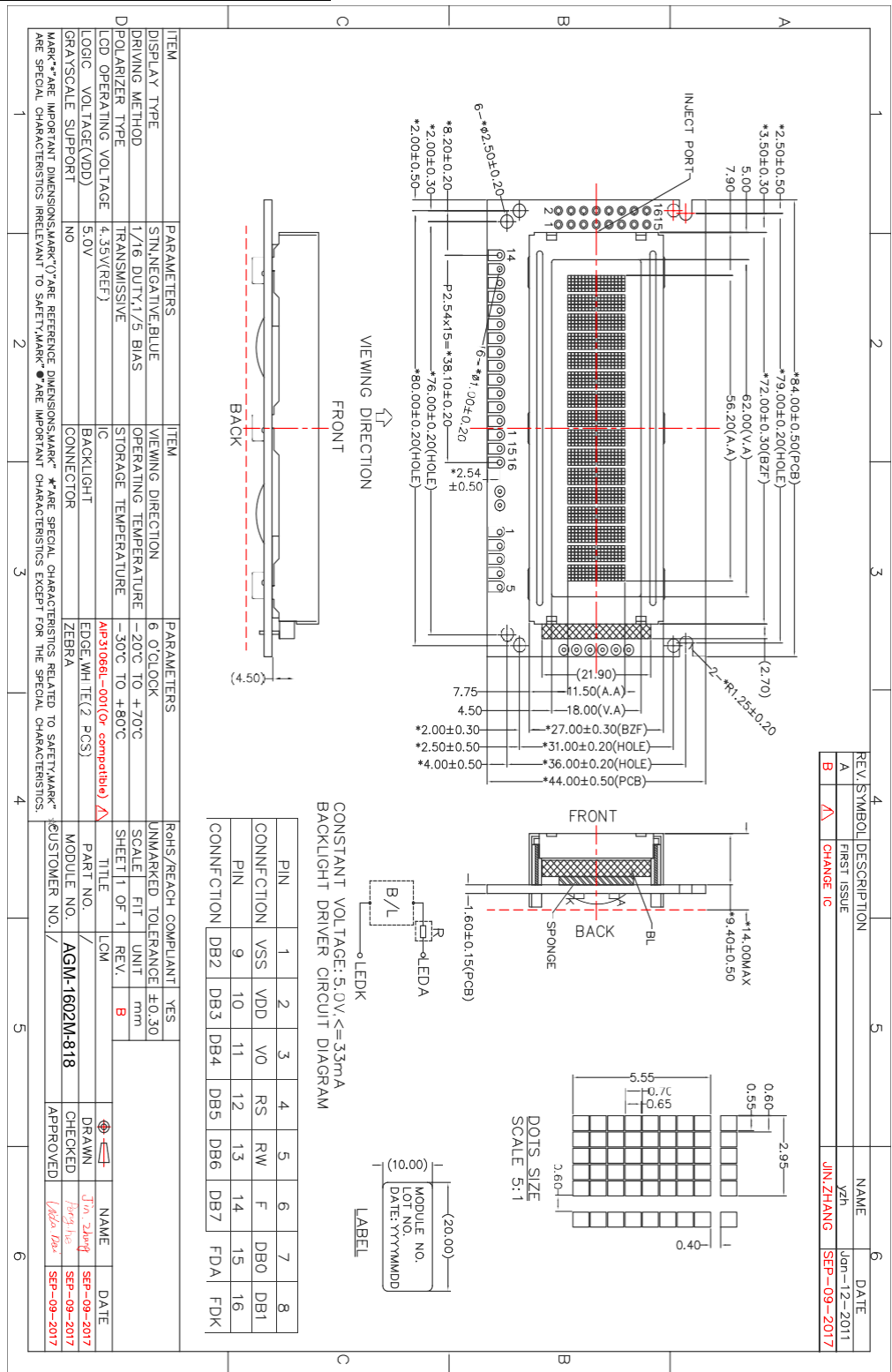
Figure 2. Dimensional outline
