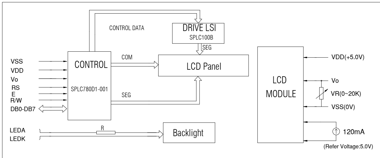
Figure 1. Block diagram
