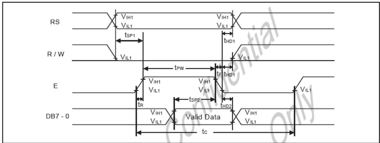
Figure 3. Write Mode Timing Diagram
