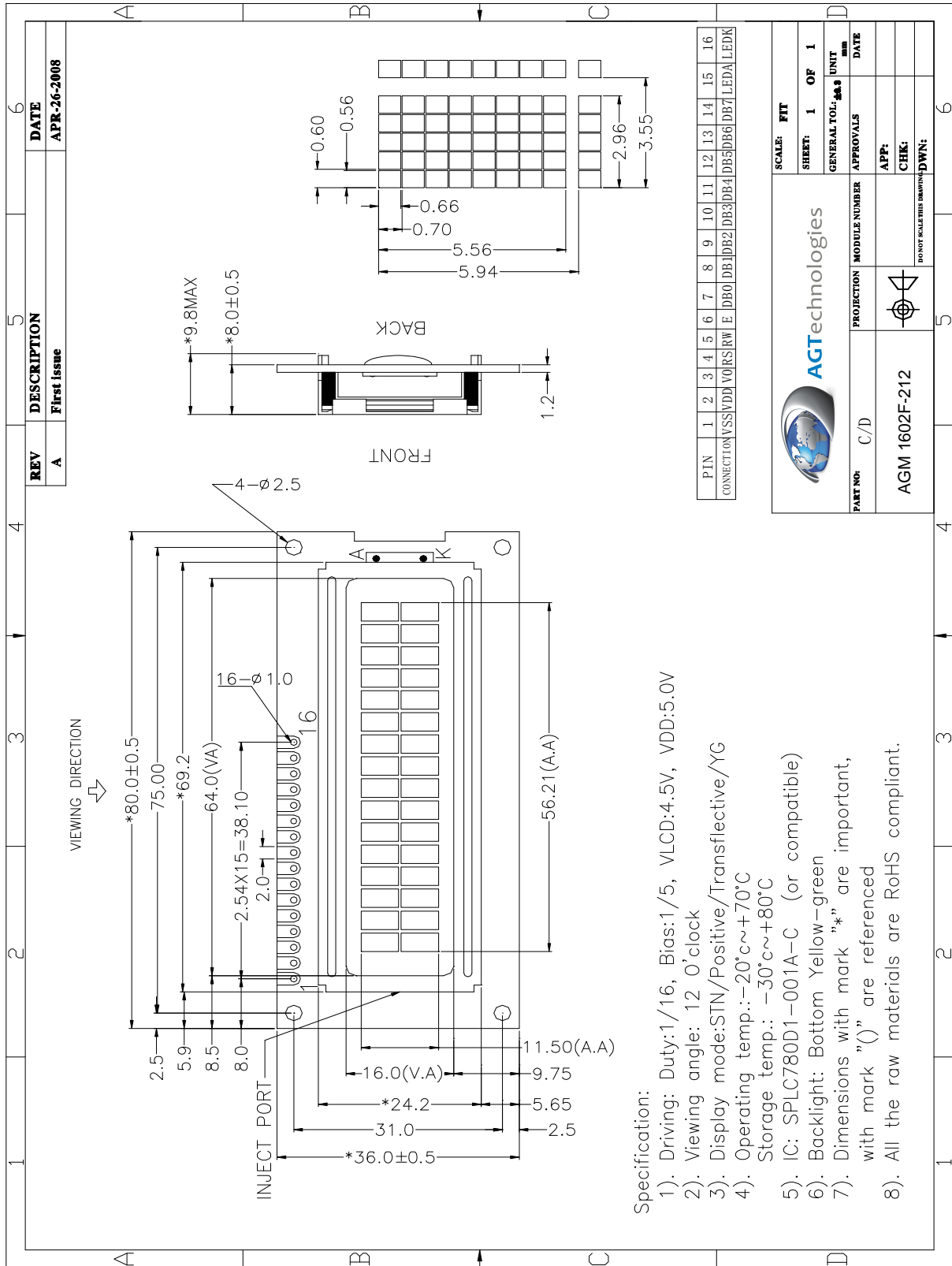
Figure 2. Dimensional outline
