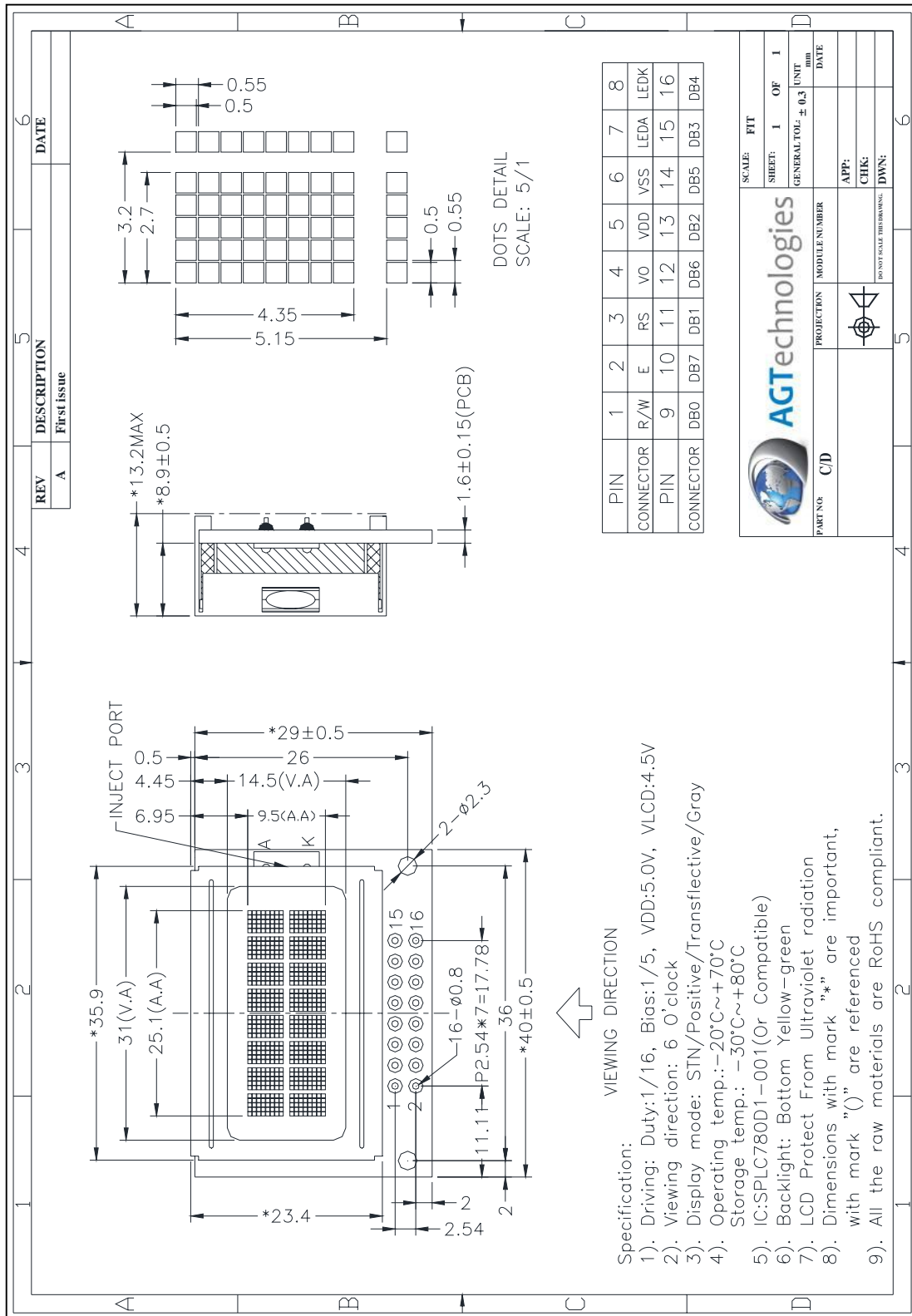
Figure 2. Dimensional outline
